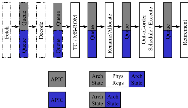
Figure 4 Intel® Xeon™ processor pipeline
