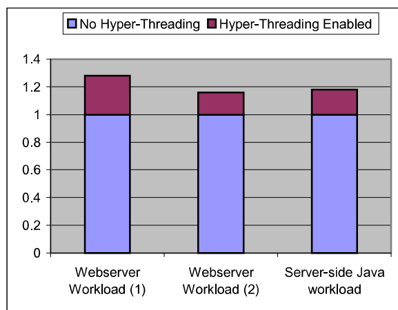
Figure 9: Web server benchmark performance
