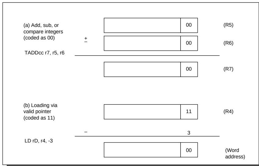
Figure I.32 SPARC uses the two least-significant bits to encode different data types for the tagged arithmetic instructions. (a) Integer arithmetic, which takes a single cycle as long as the operands and the result are integers. (b) The misaligned trap can be used to catch invalid memory accesses, such as trying to use an integer as a pointer. For languages with paired data like LISP, an offset of -3 can be used to access the even word of a pair ( CAR ) and +1 can be used for the odd word of a pair ( CDR ).
