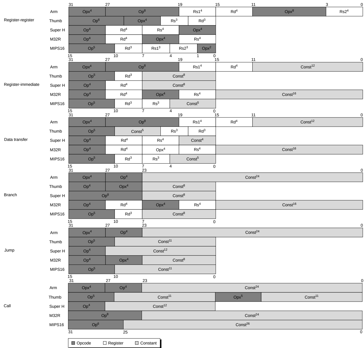
Figure I.6 Instruction formats for embedded RISC architectures. These six formats are found in all five architectures. The notation is the same as Figure I.5. Note the similarities in branch, jump, and call formats, and the diversity in register-register, register-immediate, and data transfer formats. The differences result from whether the architecture has 8 or 16 registers, whether it is a 2- or 3-operand format, and whether the instruction length is 16 or 32 bits.
