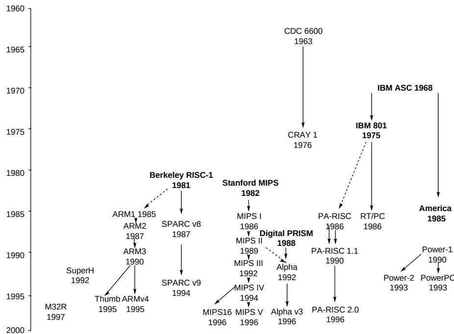
Figure I.35 The lineage of RISC instruction sets. Commercial machines are shown in plain text and research machines in bold. The CDC-6600 and Cray-1 were load-store machines with register 0 fixed at 0, and separate integer and floating-point registers. Instructions could not cross word boundaries. An early IBM research machine led to the 801 and America research projects, with the 801 leading to the unsuccessful RT/PC and America leading to the successful Power architecture. Some people who worked on the 801 later joined Hewlett Packard to work on the PA-RISC. The two university projects were the basis of MIPS and SPARC machines. According to Furber [1996], the Berkeley RISC project was the inspiration of the ARM architecture. While ARM1, ARM2, and ARM3 were names of both architectures and chips, ARM version 4 is the name of the architecture used in ARM7, ARM8, and StrongARM chips. (There are no ARMv4 and ARM5 chips, but ARM6 and early ARM7 chips use the ARM3 architecture.) DEC built a RISC microprocessor in 1988 but did not introduce it. Instead, DEC shipped workstations using MIPS microprocessors for three years before they brought out their own RISC instruction set, Alpha 21064, which is very similar to MIPS III and PRISM. The Alpha architecture has had small extensions but they have not been formalized with version numbers; we used the version 3 because that is the version of the reference manual. The Alpha 21164A chip added byte and halfword loads and stores, and the Alpha 21264 includes the MAX multimedia and bit count instructions. Internally, Digital names chips after the fabrication technology: EV4 (21064), EV45 (21064A), EV5 (21164), EV56 (21164A), and EV6 (21264). "EV" stands for "extended VAX."
