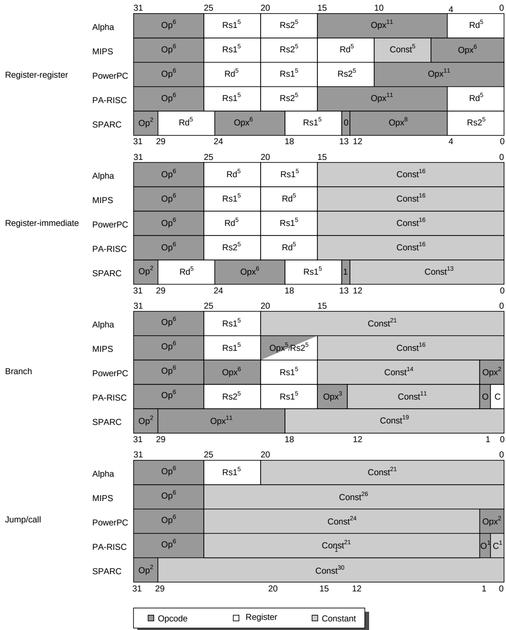
Figure I.5 Instruction formats for desktop RISC architectures. These four formats are found in all five architectures. (The superscript notation in this figure means the width of a field in bits.) Although the register fields are located in similar pieces of the instruction, be aware that the destination and two source fields are scrambled. Op = the main opcode, Opx = an opcode extension, Rd = the destination register, Rs1 = source register 1, Rs2 = source register 2, and Const = a constant (used as an immediate or as an address). Unlike the other RISCs, Alpha has a format for immediates in arithmetic and logical operations that is different from the data transfer format shown here. It provides an 8-bit immediate in bits 20 to 13 of the RR format, with bits 12 to 5 remaining as an opcode extension.
