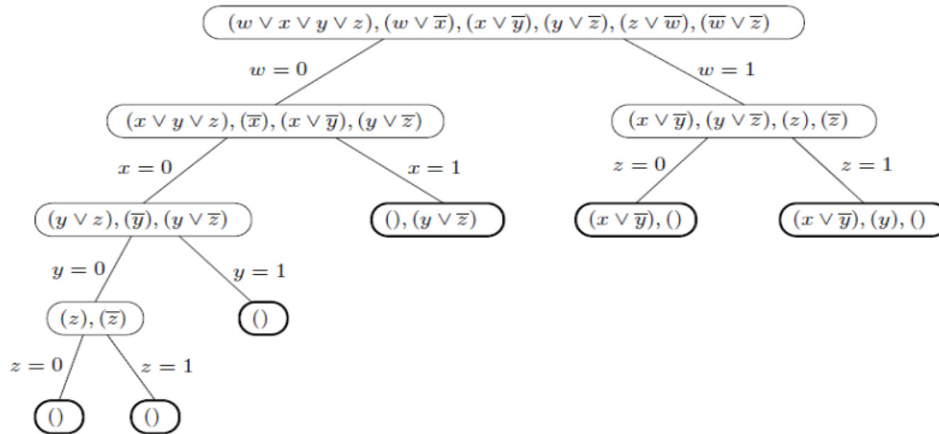
Figure 9.1 Backtracking reveals that \phi is not satisfiable.
